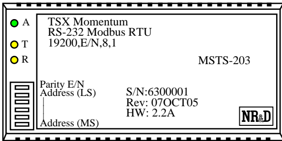
Figure 1 MSTS-203 Layout
