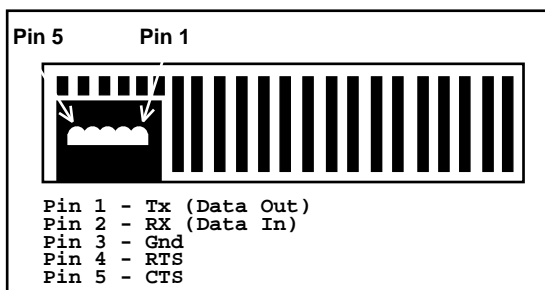
Figure 3 5-Pin RS-232 Port
