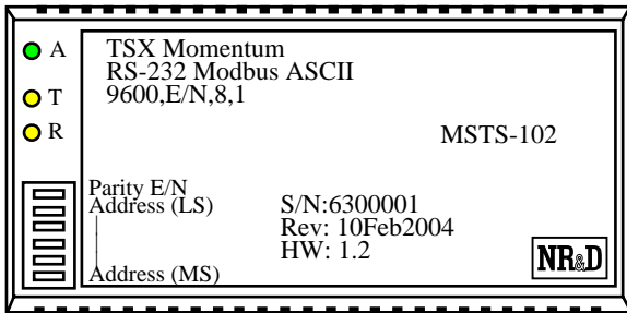
Figure 1 MSTS-102 Layout
