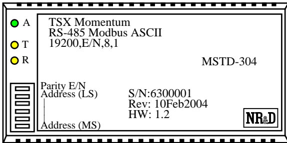
Figure 1 MSTD-304 Layout
