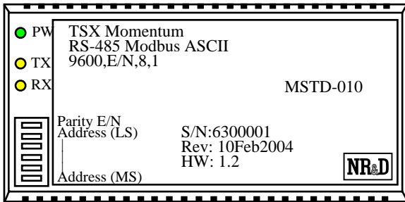
Figure 1 MSTD-010 Layout
