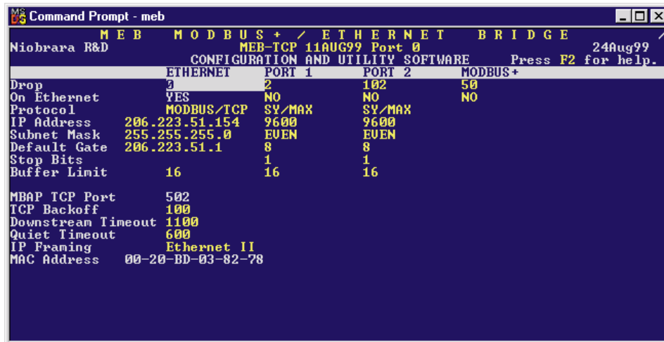
Figure 24-3 MEBSW32 online Edit Screen
