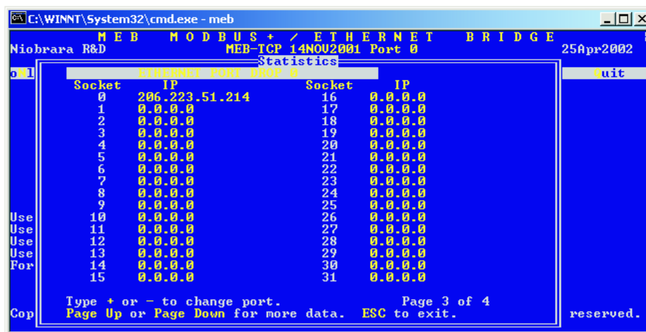
Figure 24-8 Ethernet Port Statistical Screen (Pages 3&4)
