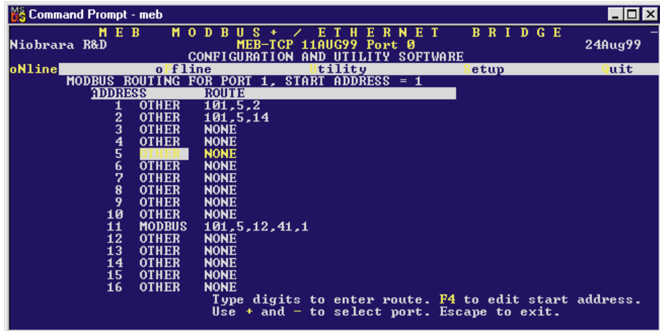
Figure 24-11 Edit Modbus Slave Routing
