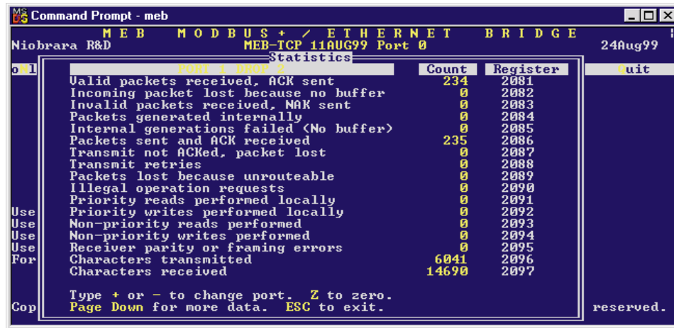
Figure 24-9 Port 1..2 Statistical Screen (Page 1)
