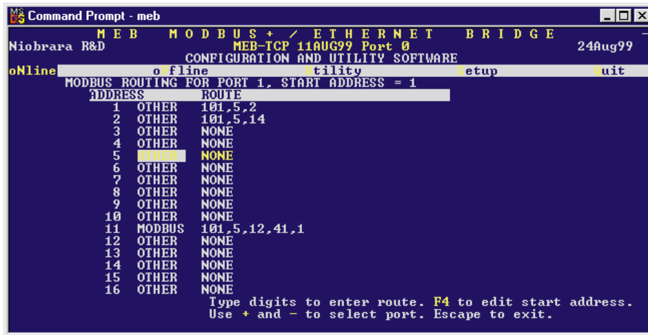
Figure 16-4 MEBSW32 Modbus Routing Editing Screen
