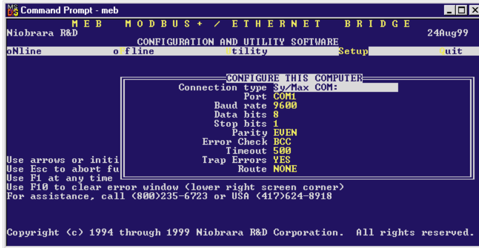
Figure 24-21 SY/MAX Setup Screen
