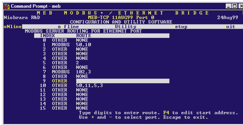
Figure 24-12 Modbus Server Routing for Ethernet Port
