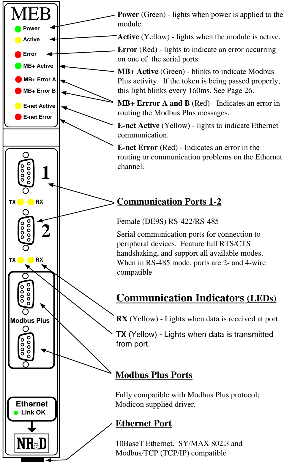
Figure 1-1 MEB-RT Front Panel
