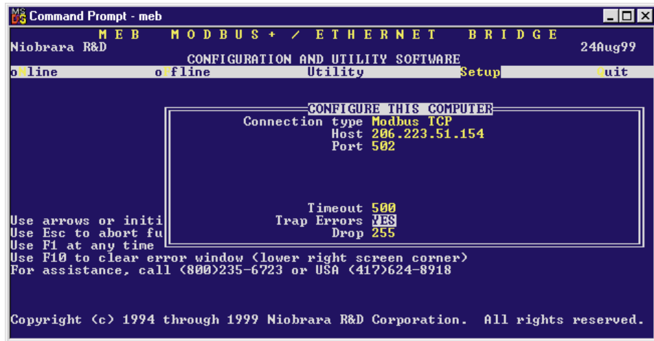
Figure 24-22 MODBUS/TCP Setup Screen
