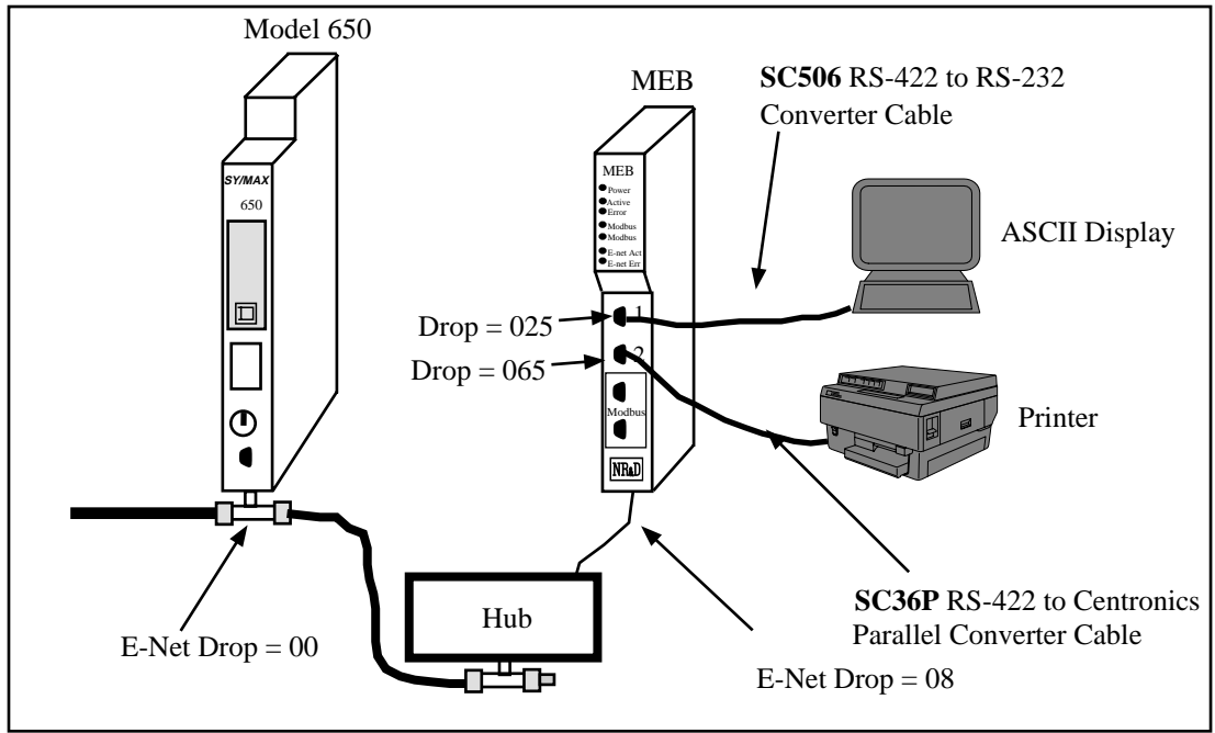
Figure 10-1 Peripheral mode example
