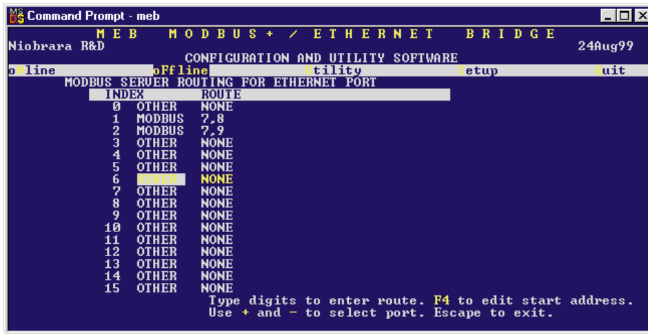
Figure 6-2 MEBSW32 Modbus Server Routing Table
