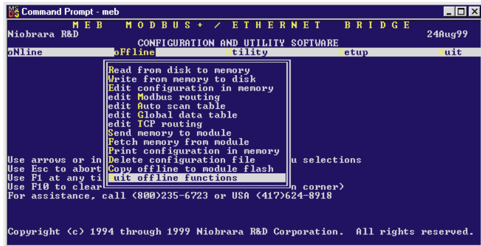
Figure 24-2 MEBSW32 offline Menu
